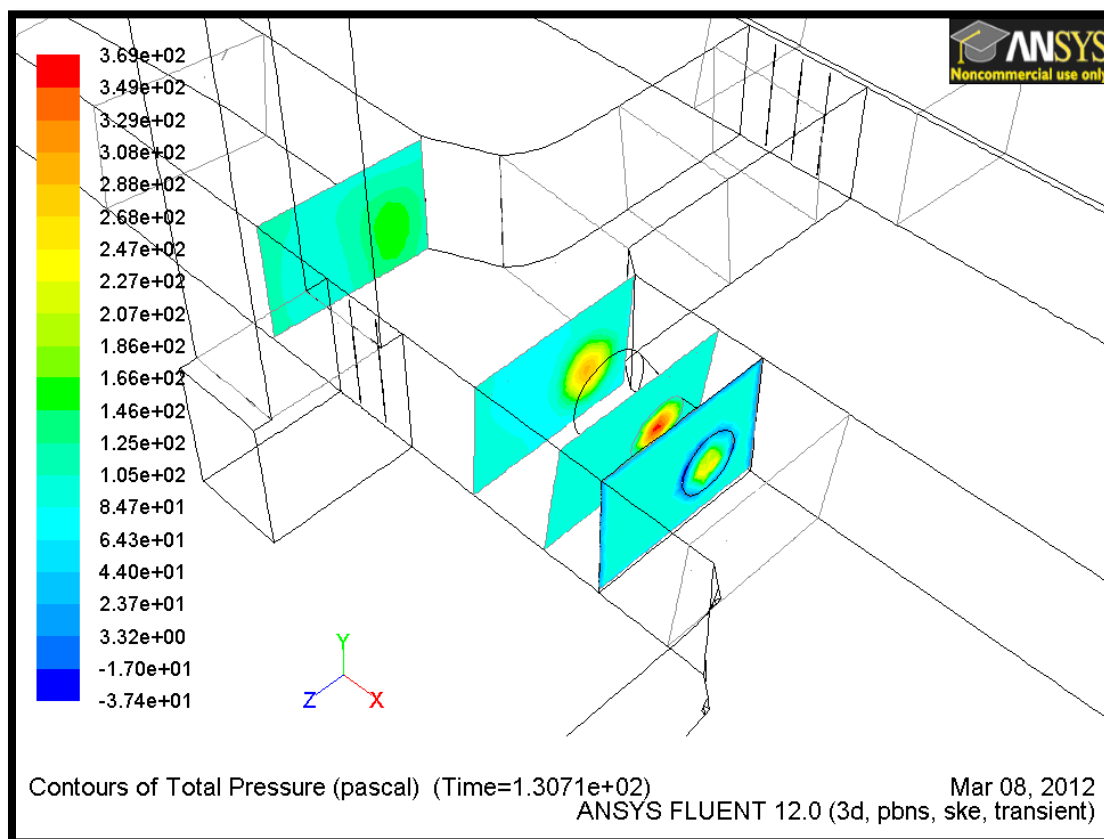
Figure 8.12. Area-weighted average total pressure downstream to the booster fan
